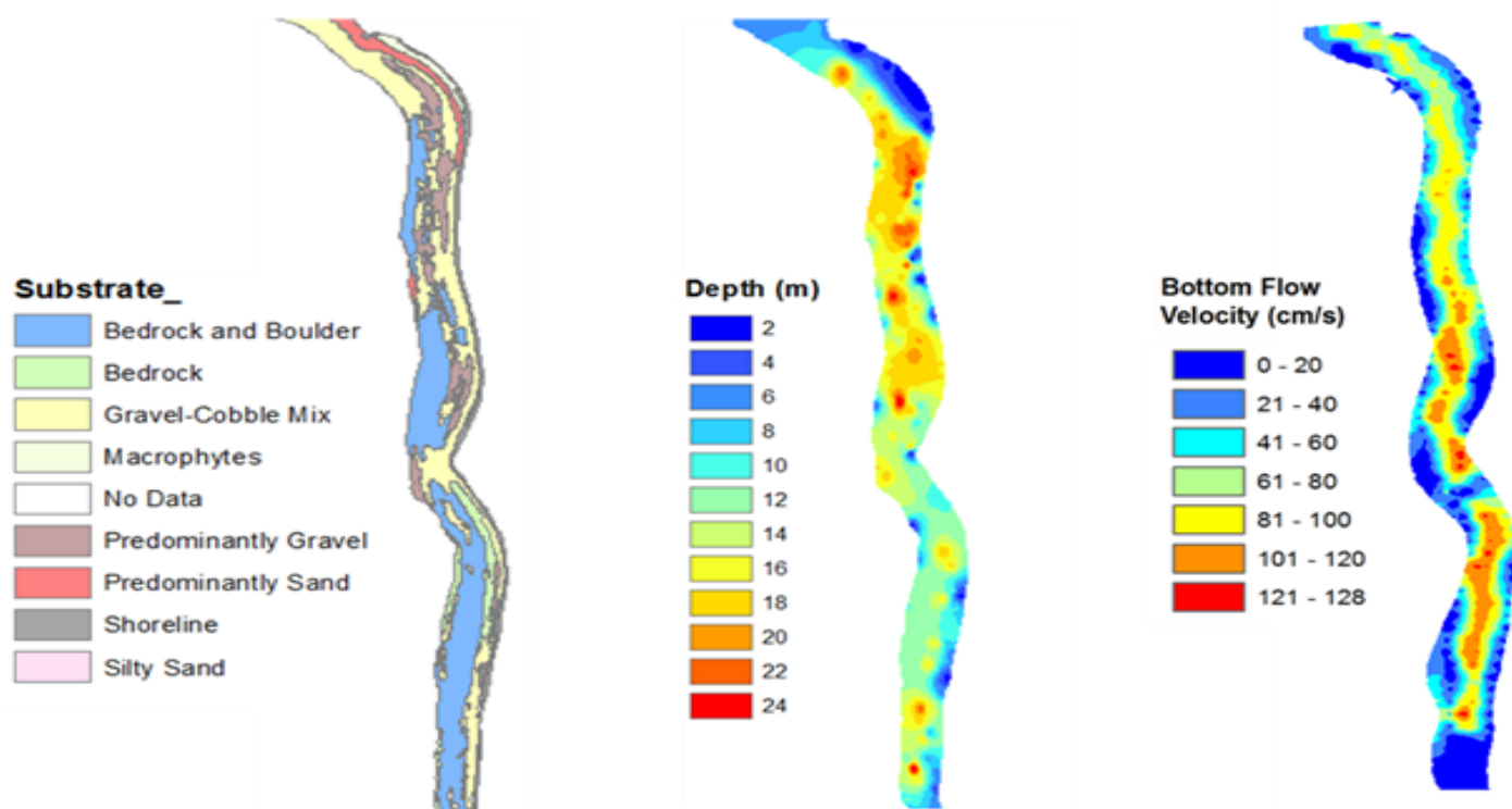
Acoustic Doppler Current Profiler data.
